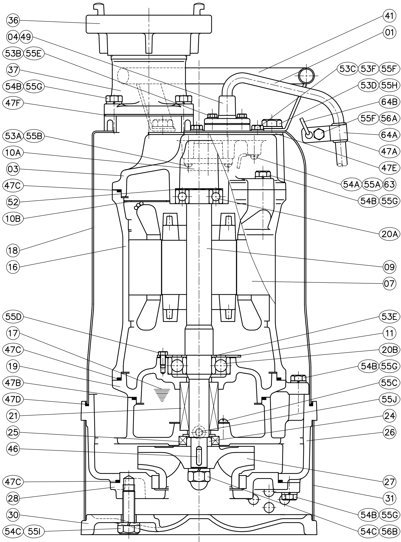
80ASN21.5 400V
